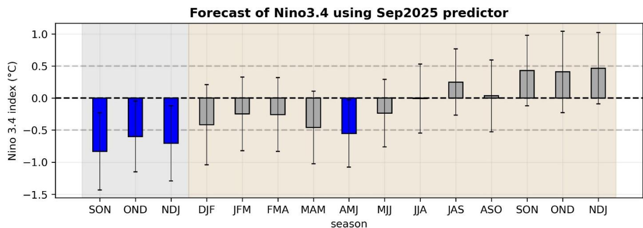
Fig. 4: Median prediction of Nino 3.4 index using July 2025-September 2025 predictors for the upcoming seasons.
