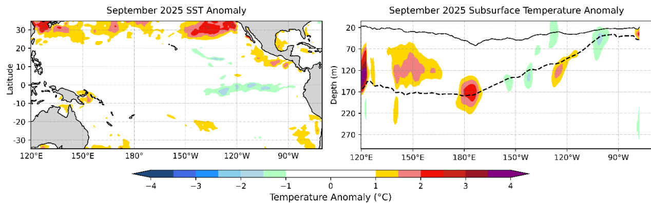
Fig. 3: (Left) Monthly SST anomaly for the tropical Pacific in September 2025. (Right) Subsurface temperature anomaly averaged over 5° S-5° N for September 2025.
