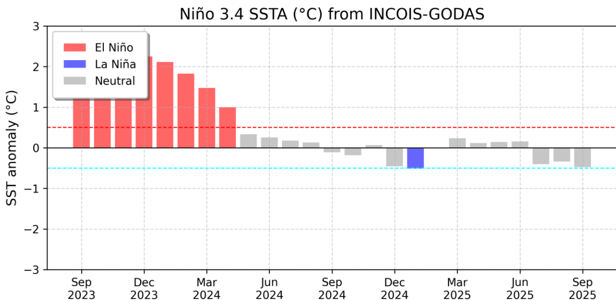
Fig. 1: Evolution of Sea Surface Temperature anomalies ( ^{\circ}\text{C} ) in the Niño 3.4 ( 5^{\circ}\text{S} - 5^{\circ}\text{N} , 170^{\circ}\text{W} - 120^{\circ}\text{W} ) region in the period September 2023- September 2025. The RED and CYAN horizontal lines represent 0.5^{\circ}\text{C} SST anomaly
